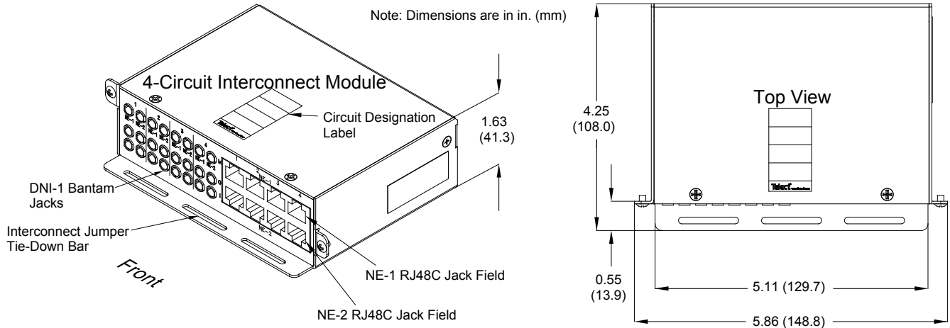
Figure 23 - Model ELF-3004-1800 Dimensions
