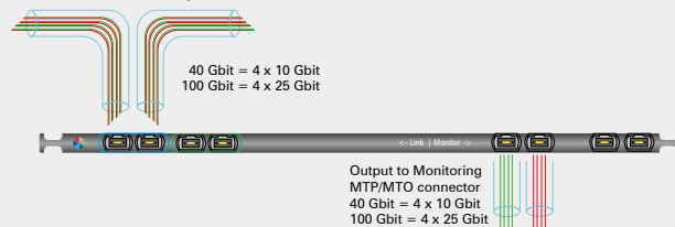
40 or 100 Gbit live link MTP/MTO connector
