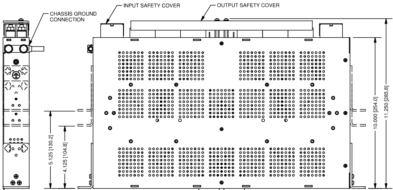
REAR VIEW ROTATED
